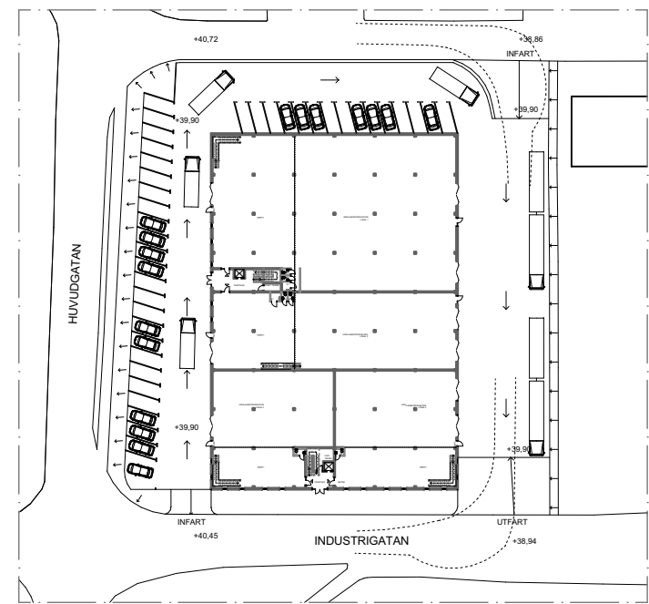
SITUATIONSPLAN
